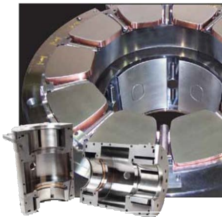
Figure 4 Horizontal bearing assemblies.
