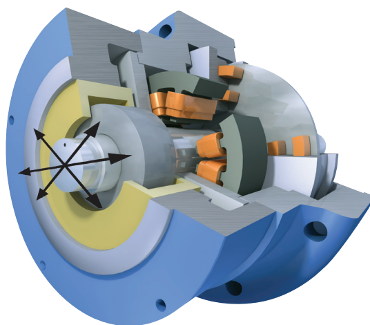
The clearance from the rotor to the stator is measured while the system is statically levitated. The clearance provides a direct measurement of the remaining auxiliary bearing service life.
