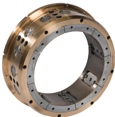
An RDS auxiliary bearing design for a large motor-compressor application.
